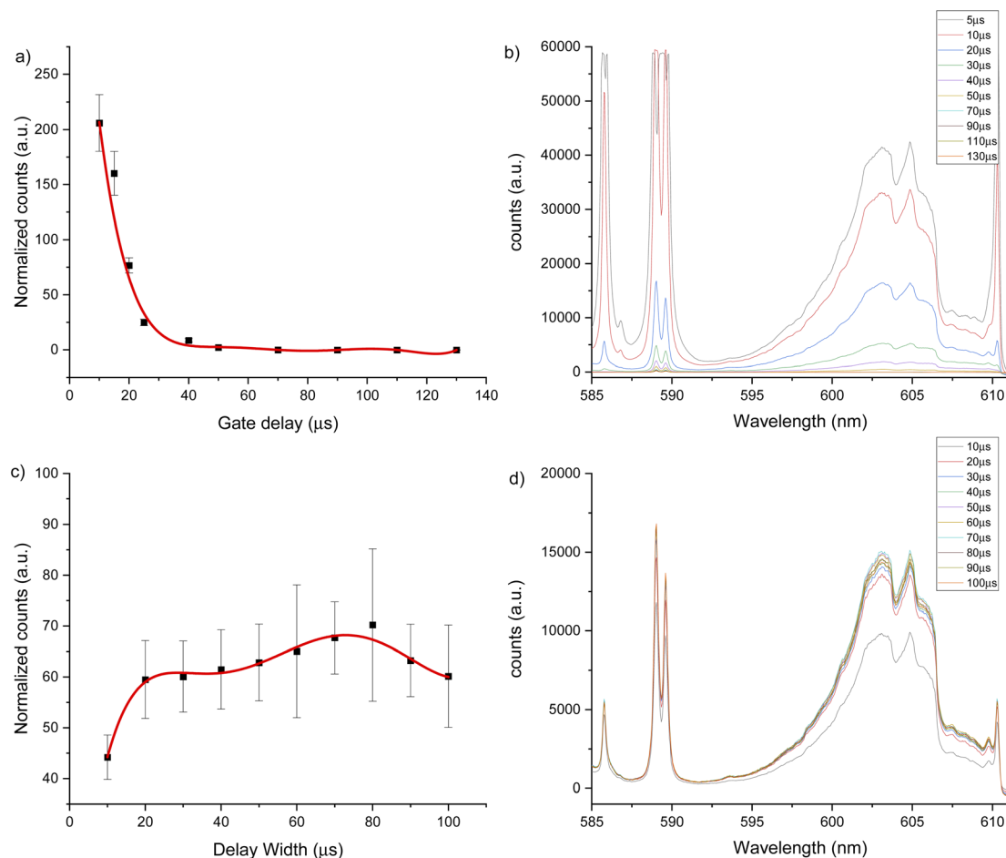
Fig. 4 LIBS signal optimization under argon flow of 1 L \text{min}^{-1} for 600 nm window using a 2500 \mu\text{g g}^{-1} hydroxyapatite standard. (a) Gate delay optimization maintaining constant gate width at 50 \mu\text{s} , (b) LIBS spectrum for each gate delay change, (c) gate width optimization maintaining constant gate delay at 20 \mu\text{s} , (d) LIBS spectrum for each gate width change.
