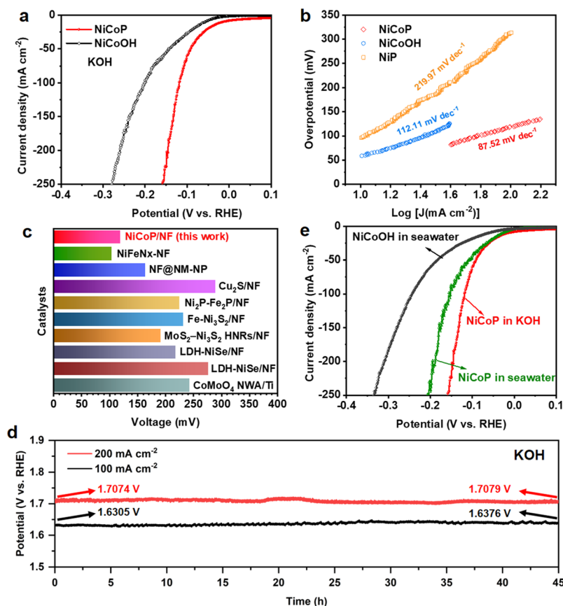
Fig. 4 (a) LSV curves and (b) the corresponding Tafel plots of NiCoOH and NiCoP electrocatalysts in 1.0 M KOH. (c) A comparison of the HER in 1.0 M KOH at a current density of 100 mA cm -2 between NiCoP and other noble-metal catalysts reported to date. (d) 45 h stability test of NiCoP for a cathodic HER at 100 and 200 mA cm -2 and (e) LSV curves of the NiCoOH and NiCoP electrocatalysts in 1.0 M KOH and alkaline seawater.
