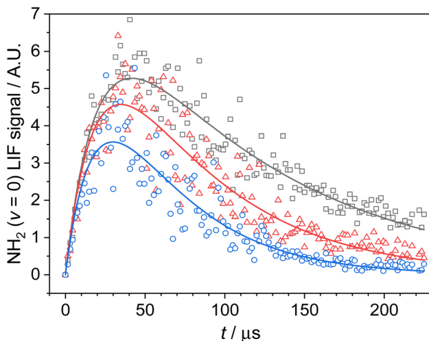
Fig. 1 \text{NH}_2 ( v = 0 ) temporal traces collected at 52.2 K, a total Ar density of 6.2 \times 10^{16} molecules per \text{cm}^3 , [\text{NH}_3] = 2.5 \times 10^{13} molecules per \text{cm}^3 , [\text{CH}_4] = 1.8 \times 10^{15} molecules per \text{cm}^3 , and [\text{CH}_3\text{CHO}] of 1.3, 2.8 and 5.1 \times 10^{14} molecules per \text{cm}^3 (grey squares, red triangles, and blue circles respectively). Solid lines are the least squares fitting of a bi-exponential function to the traces from which k'_{\text{obs}} is obtained (see Section 3.1 for details).
