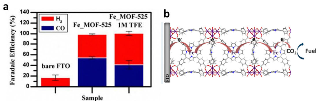
Fig. 19 (a) FE over approximately 4 h of bare FTO, Fe 2 MOF-525 with/without 2,2,2-trifluoroethanol (TFE). (b) Proposed ECR mechanism on the Fe porphyrin-based MOF. Reproduced with permission. 22 Copyright (2015) American Chemical Society.
