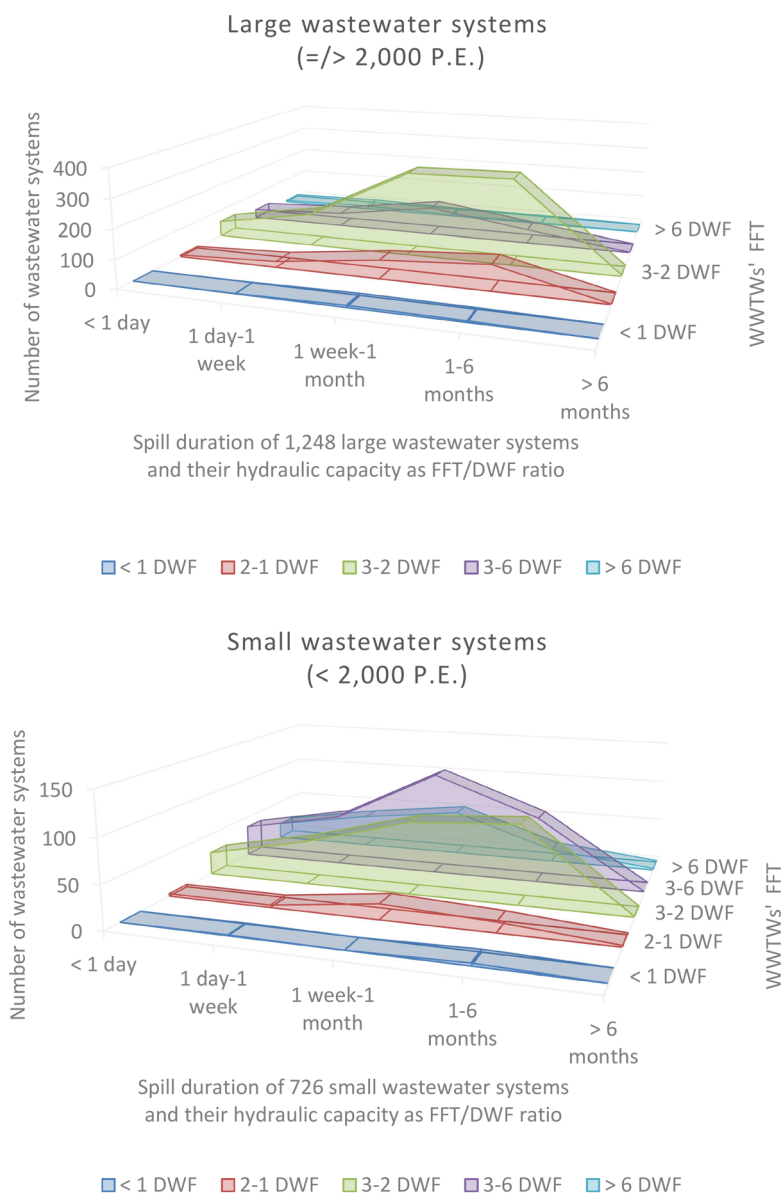
Fig. 3 Spill duration of wastewater systems during 2021 and the flow to full treatment (FFT) of their wastewater treatment works (WWTWs) expressed as multiples of dry weather flow (DWF) in five categories: spilled up to a day ( \leq 1 d); spilled between a day and a week (1 d–1 w); spilled between a week and 1 month (1 w–1 m); spilled between 1 and 6 months (1 m–6 m); and spilled more than 6 months ( > 6 m).
