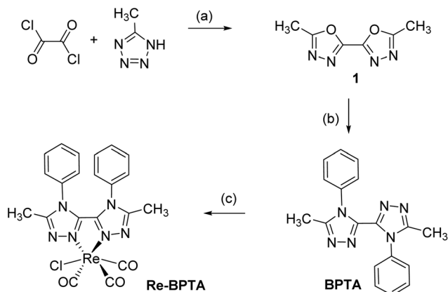
Fig. 1 Chemical structures of the SLE-active tricarbonylrhenium(i) complexes previously studied (ref. 25–29) and of the new Re-BPTA complex.
