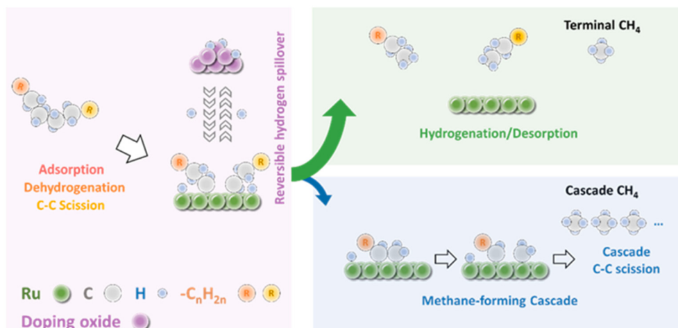
Fig. 5 Schematic of the mechanism for LDPE hydrogenolysis. Reproduced from ref. 57 with permission from Elsevier.
