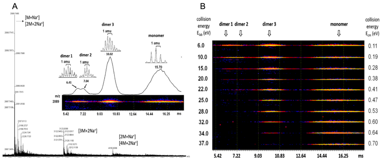
Fig. 4 (A) ESI MS of (BPOSS-PDI-C 60 ). (B) 2D TWIM-MS plot of dimer and monomers present and their dissociation energies. Reproduced/adapted from ref. 57 with permission from MDPI Molecules .
