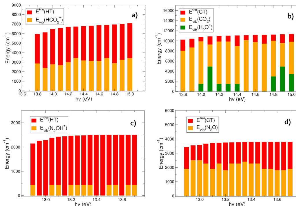
Fig. 6 Energy content of the products formed in the reaction involving CO 2 + + H 2 O in HT (a) and CT channels (b). Energy content of the products formed in the reaction involving N 2 O + + H 2 O in HT (c) and CT channels (d).
