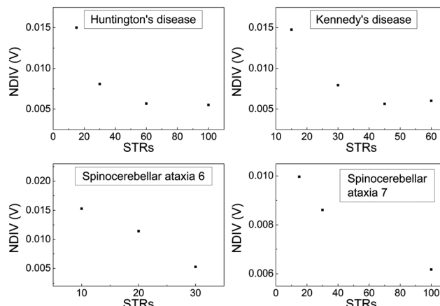
Fig. 18 Normalised deviation of the I-V curve from the origin (NDIV) as a function of the number of (CAG) repeats aka short tandem repeat (STR) expansions. Upper left panel: Huntington's disease, upper right panel: Kennedy's disease, left lower panel: Spinocerebellar ataxia 6, lower right panel: Spinocerebellar ataxia 7.
