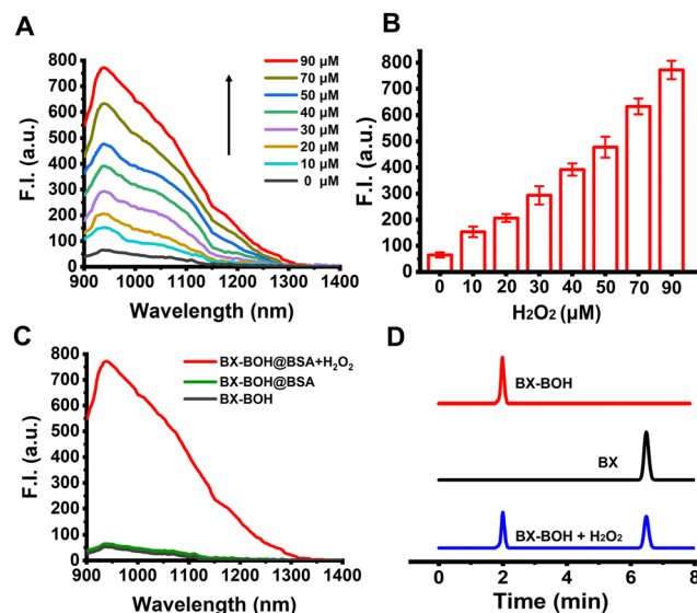
Fig. 1 (A) NIR-II fluorescence spectra for BX-BOH@BSA ( 0.6 \text{ mg mL}^{-1} ) without and with incubation with H_2O_2 in PBS (with 5% DMSO, pH 7.4). (B) Fluorescence intensity at 938 nm for BX-BOH@BSA ( 0.6 \text{ mg mL}^{-1} ) without or with incubation with H_2O_2 in PBS (with 5% DMSO, pH 7.4) ( n = 3 ). (C) NIR-II fluorescence spectra of BX-BOH, BX-BOH@BSA and BX-BOH@BSA + H_2O_2 upon reaction with H_2O_2 (90 \mu M), respectively. (D) HPLC chromatograms for BX-BOH, BX, and BX-BOH were treated with H_2O_2 for 40 min (MeOH is the mobile phase with 1.0 \text{ mL min}^{-1} flow rate).
