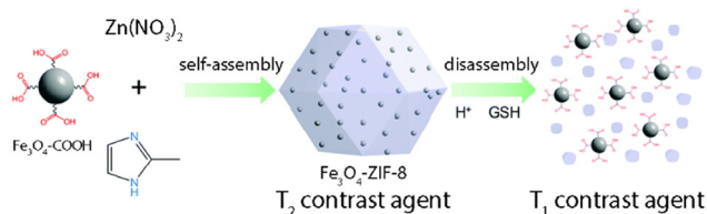
Fig. 17 \text{T}_1 - \text{T}_2 responsive \text{Fe}_3\text{O}_4@ZIF-8 nanosystem assembly and disassembly triggered by pH and glutathione (GSH). Adapted from ref. 132.
