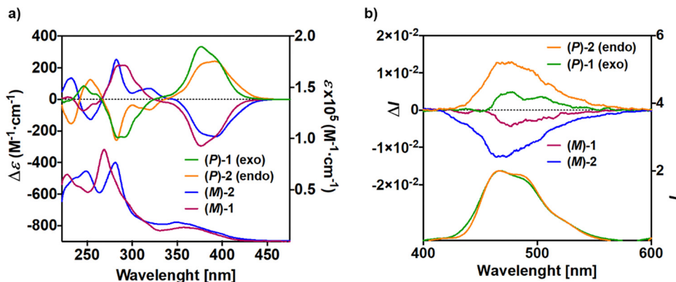
Fig. 2 (a) Experimental UV-vis (bottom) and ECD (top) spectra and (b) fluorescence (bottom) and CPL (top) spectra of (P) and (M) enantiomers of 1 and 2 ( CH_2Cl_2 , C \sim 10^{-5} M).
