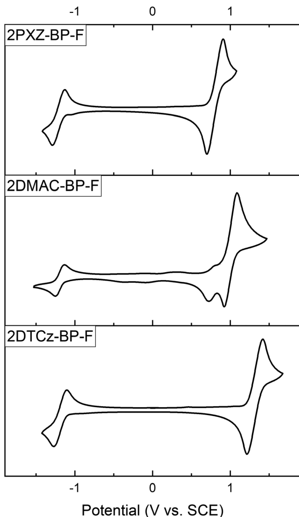
Fig. 4 Cyclic voltammograms of 2PXZ-BP-F , 2DMAC-BP-F , and 2DTCz-BP-F in Ar-saturated DCM solution (0.1 M [ n Bu 4 N][PF 6 ]) at a scan rate of 100 mV s -1 .
