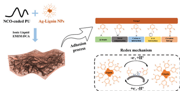
Fig. 1 Design strategy and mechanism of the self-adhesive ionogel.
