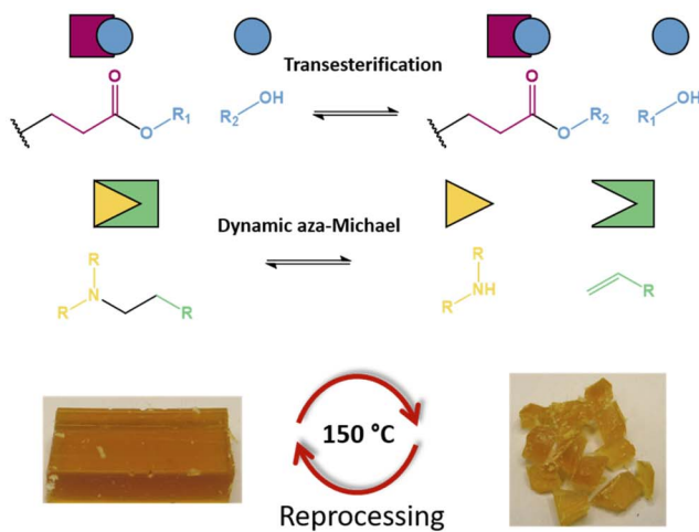
Fig. 6 Schematic representations of BAE-F-OH, BAE-F and BAE-OH associated with their respective exchange reactions and reprocessing conditions.
