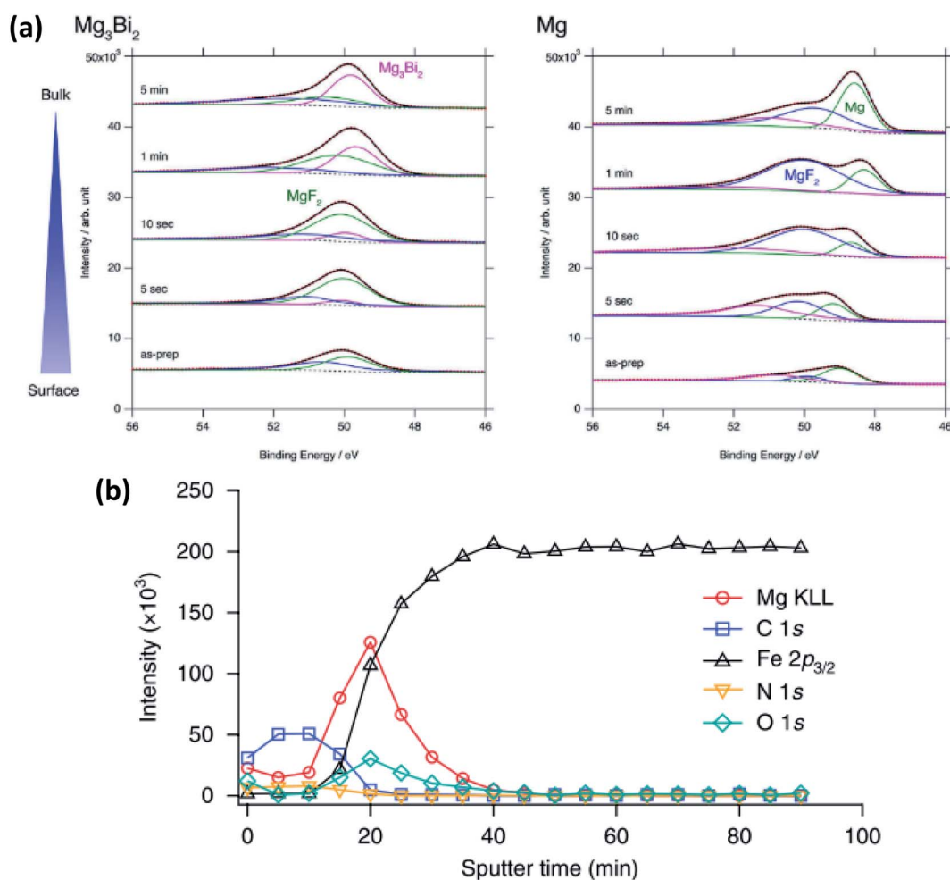
Fig. 18 (a) Mg 2p XPS spectra after sputter-etch depth profiling for \text{Mg}_3\text{Bi}_2 and Mg thin films immersed in 0.5 mol L −1 Mg(TFSa) 2 in BuMeG3 solution for 24 h. Reproduced under CC-BY licence from ref. 155. (b) XPS sputter-etch depth profiles of a Mg-coated stainless-steel electrode in 0.5 M Mg(TFSI) 2 -PC electrolyte. Reprinted by permission from Nature Chemistry 156 Copyright 2018.
