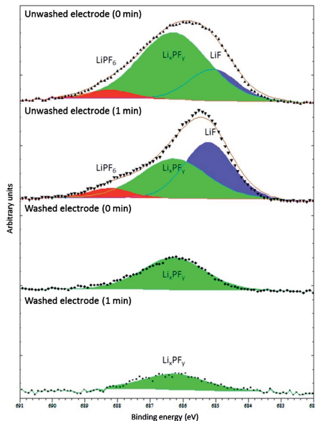
Fig. 6 F 1s XPS spectra (Al K\alpha , 1487 eV) from washed (dimethyl carbonate (DMC), 2 min, dried in argon) and unwashed graphite anode from full cells with \text{LiCoO}_2 cathode and electrolyte of 1 M \text{LiPF}_6 in ethylene carbonate (EC)/ethyl methyl carbonate (EMC), 3 : 7 w/w. The minutes in the figure refer to the duration of \text{Ar}^+ sputtering before XPS measurement. Reproduced under CC-BY licence from ref. 66.
