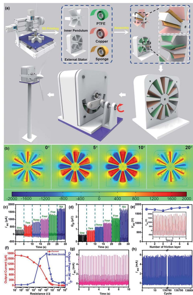
Fig. 2 (a) The schematic structure and fabrication process of the PMLA-TENG. (b) The potential distributions of different angles simulated by COMSOL. Functional parameters (c) I_{SC} , (d) Q_{tr} , and (e) V_{OC} of the PMLA-TENG with different pairs of friction layers. (f) The relationship between the loading resistance, instantaneous current and power density of the TENG with six friction layers. (g) I_{SC} after processing by a transformer and a rectifier. (h) The I_{SC} processed by a transformer and a rectifier after about 136 800 cycles (working continuously for 6 h). Reproduced with permission. 59 Copyright 2019, Elsevier.
