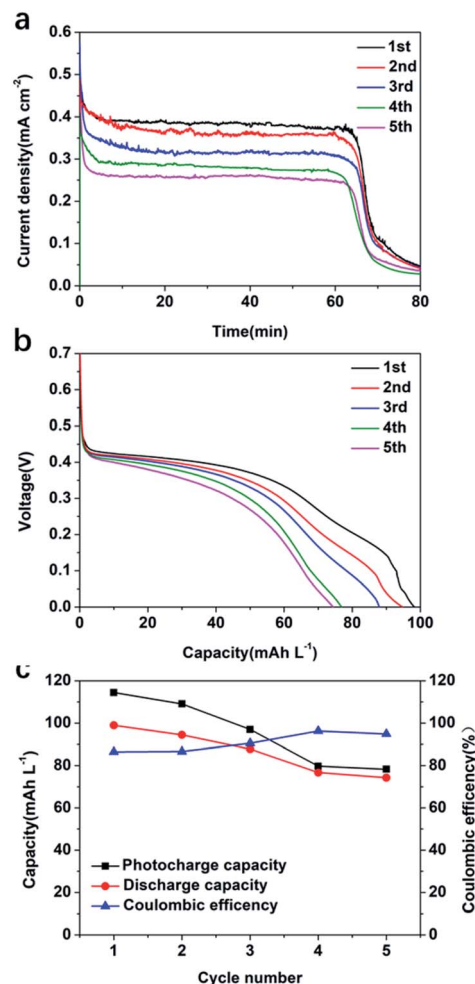
Fig. 6 (a) Cyclic photocharge and (b) discharge of \text{MoS}_2/\text{TiO}_2\text{-}0.5 and (c) the capacity and coulombic efficiency at a vanadium ion concentration of 1.0 \text{ M V}^{4+} . The discharge current density is 0.4 \text{ mA cm}^{-2} ( 100 \text{ mW cm}^{-2} (AM 1.5G) with 3.0 \text{ M H}_2\text{SO}_4 and a 2.5 \text{ mL min}^{-1} flow rate).
