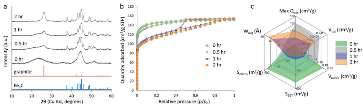
Fig. 9 (a) XRD data, (b) \text{N}_2 adsorption/desorption isotherms and (c) porosimetry data for carbons prepared by pyrolyzing starch and \text{Fe}(\text{NO}_3)_3 to 800^\circ\text{C} for various hold-times. Figure reproduced with permission from ref. 108.
