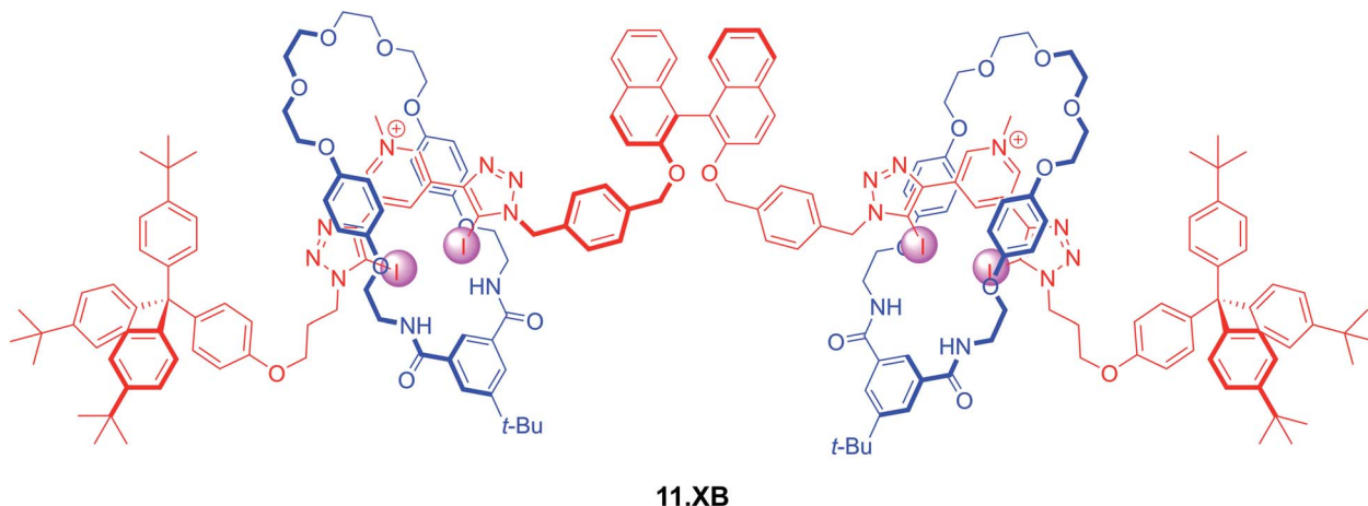
Fig. 14 S -BINOL-based fluorescent [3]rotaxane 11.XB for fluorescent discrimination of S / R -glutamate enantiomers and fumarate/maleate geometric dicarboxylate isomers in \text{CHCl}_3/\text{MeOH}/\text{H}_2\text{O} 60 : 39 : 1.
