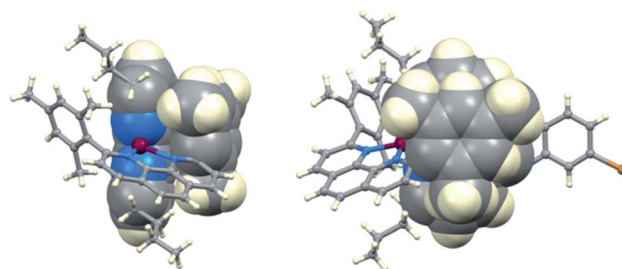
Fig. 11 Two views of the structure of a [\text{Cu}(51)(\text{phenazine})]^+ derivative (CSD refcode RNAFAP) showing the \pi -stacking interaction between one mesityl group and the phen unit of the second ligand.
