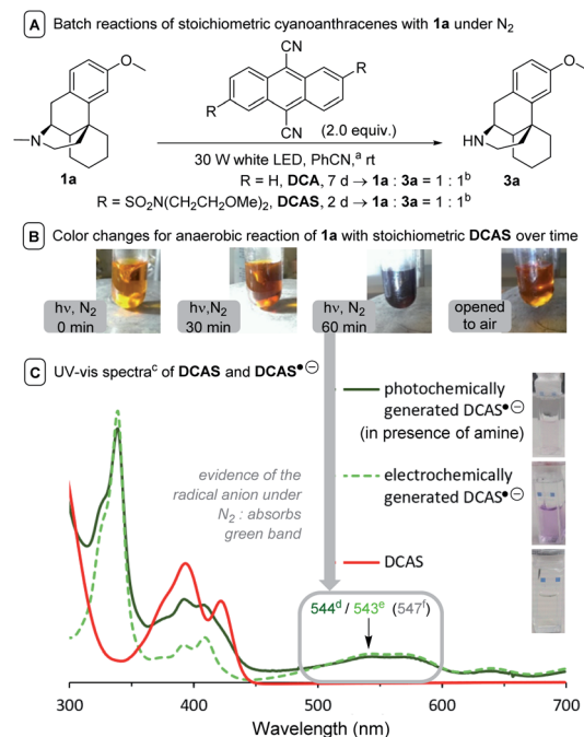
Fig. 6 Experiments suggesting the generation of cyanoanthracene radical anions. (A) Due to stoichiometric PC loadings, \text{PhCN} was chosen as solvent for improved solubility. 52 In the absence of additional base, 1a deprotonates 1a^{\bullet+} to afford 1a^{\bullet-} , meaning the reaction fundamentally could never exceed 50% conversion. (B) Observed color changes. (C) In \text{MeCN} , \lambda_{\text{max}} at the visible region when generated by photochemical reductive quenching of {}^1\text{DCAS}^* with a trialkylamine; generated electrochemically; or calculated using TD-DFT at CAM-B3LYP/6-31++g(2d,p), CPCM( \text{MeCN} ) level of theory (for details, see ESI†).
