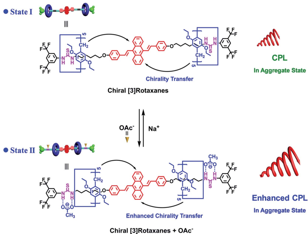
Fig. 14 Mechanism for the switchable circularly polarized luminescence (CPL) system based on the AIE-active chiral [3]rotaxanes 26 . Reprinted from ref. 75 with permission. Copyright 2021 Wiley-VCH.
