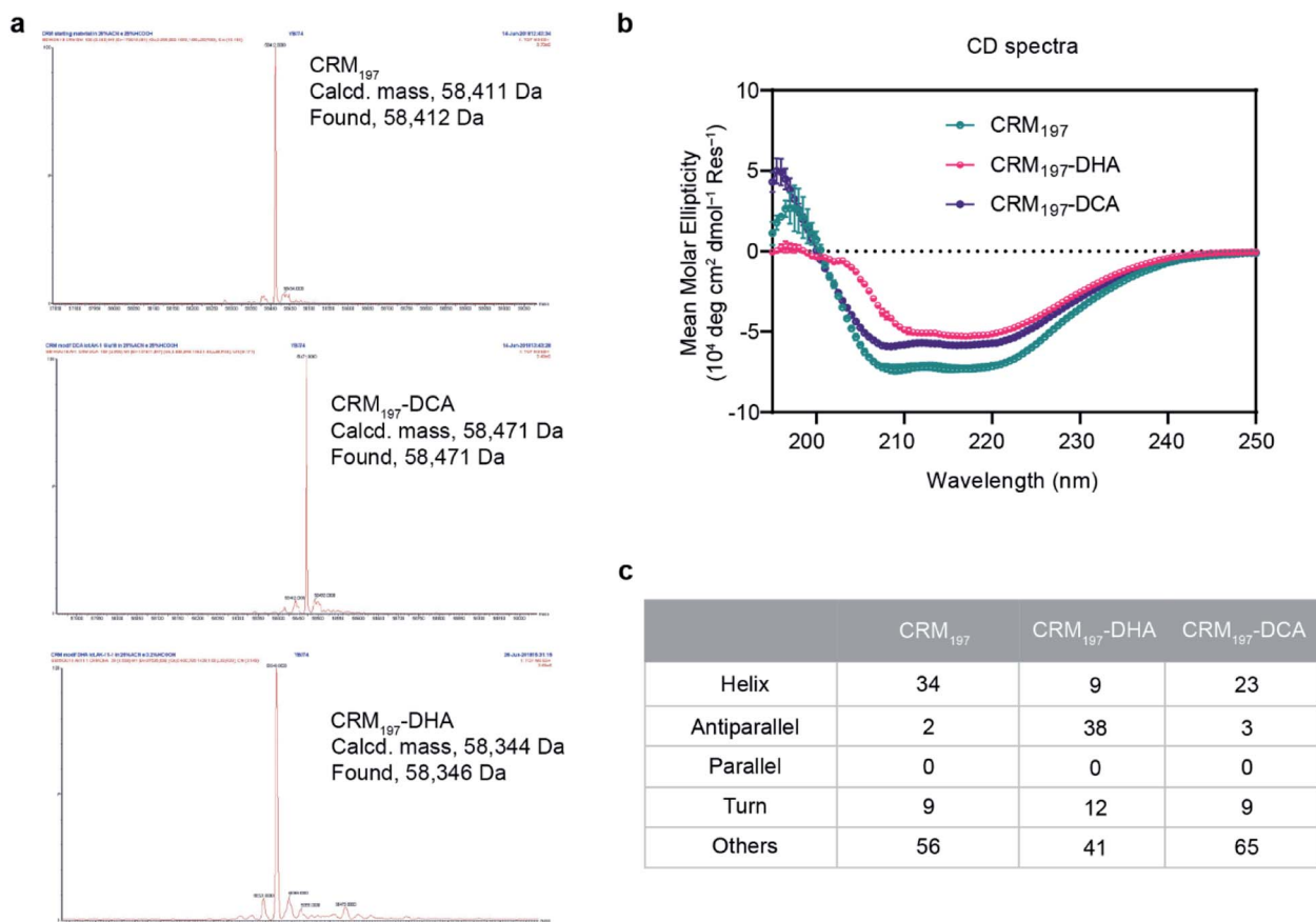
Fig. 1 A) LC-MS spectra of native CRM 197 and the modified CRM 197 -DCA and CRM 197 -DHA highlight complete conversion of native protein. (B) Secondary structure of CRM 197 , CRM 197 -DHA and CRM 197 -DCA (5 μM) determined by circular dichroism. CD spectra were obtained in phosphate buffer, pH 7.4 at 25 °C. All the values are mean values ± SEM from at least two independent experiments. (C) Estimated secondary structure content (%) from CD spectra using the BeStSel server.
