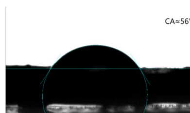
Fig. 3 The contact angle of water on the surface of Poly(VBS-DVB)HSO 4 .
