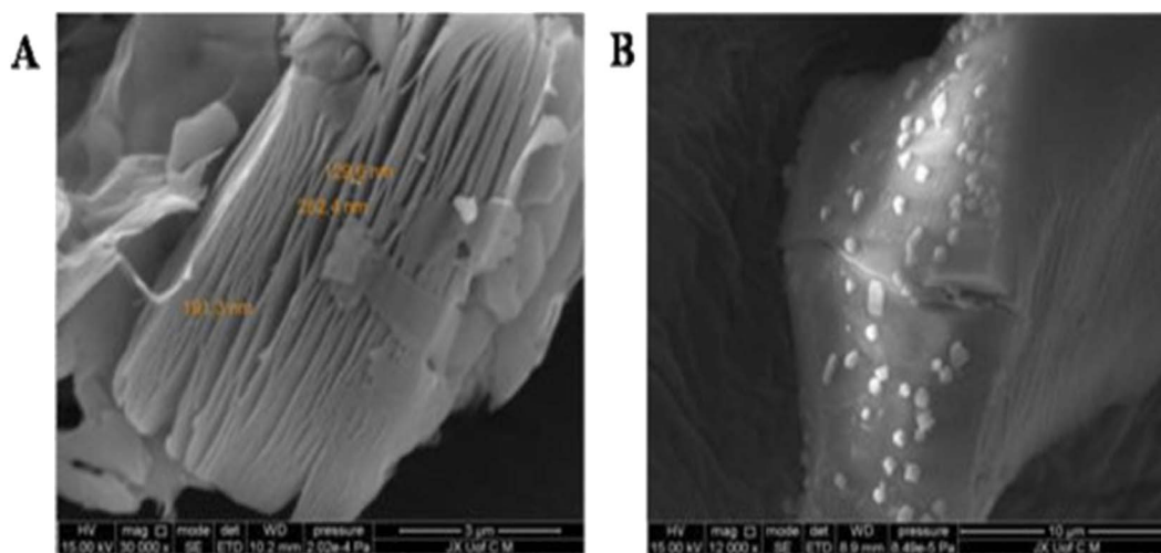
Fig. 7 SEM images of (A) pristine Ti_3C_2 and (B) Ti_3C_2-SO_3H . 78
