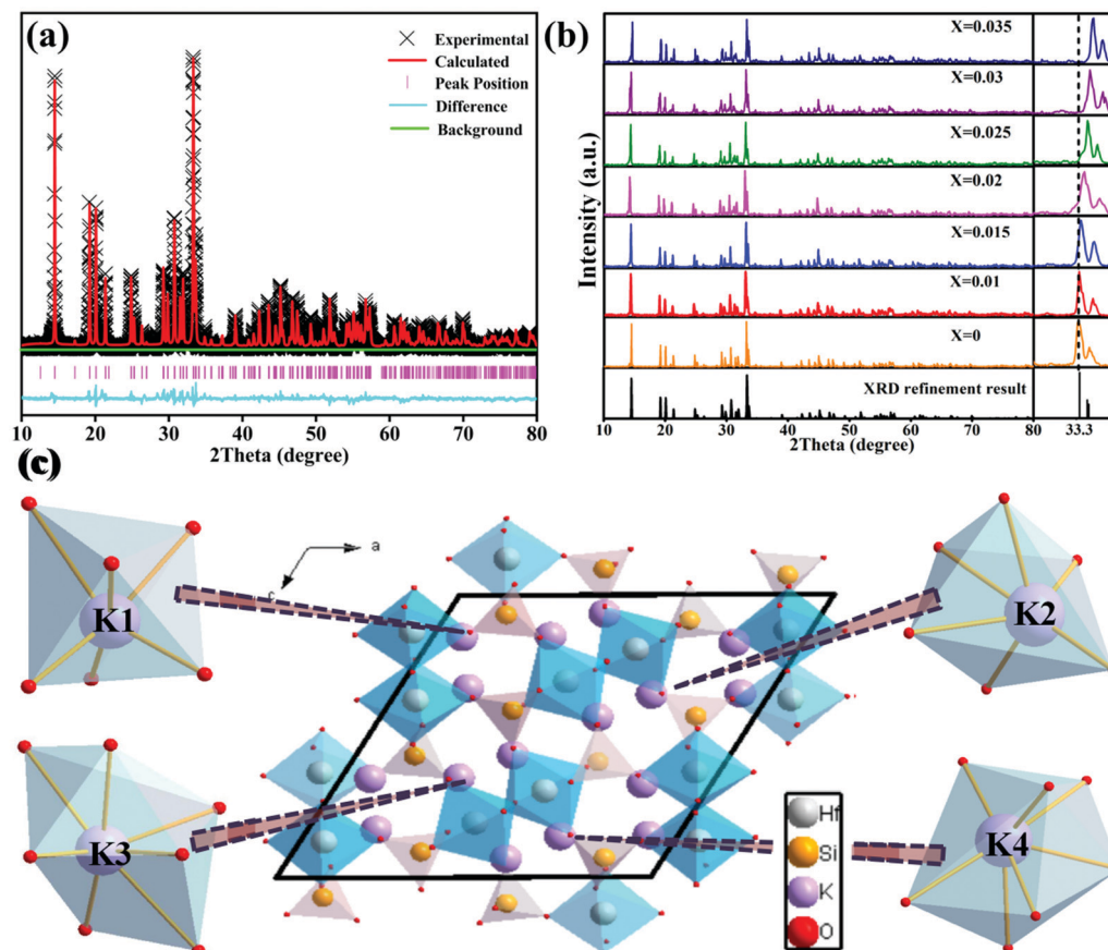
Fig. 1 (a) The \text{K}_2\text{HfSiO}_5 host Rietveld refinement result; (b) XRD patterns of \text{K}_2\text{HfSiO}_5:\text{xEu}^{2+} ( 0.00 \leq x \leq 0.035 ); and (c) the crystal structure sketch map of \text{K}_2\text{HfSiO}_5 and the different coordination surroundings of \text{K}^+ .
