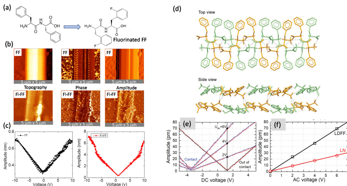
Fig. 3 Piezoelectric properties. (a) Chemical structure of FF and fluorine substituted FF (2-fluoro-L-phenylalanine-2-fluoro-L-phenylalanine) (FI-FF). (b) Topography, phase, and amplitude images of FF and FI-FF. (c) Local DC voltage amplitude loops (piezoelectric response) from FF and FI-FF tubes at an AC voltage of 0.5 V. Reprinted with permission from ref. 65, copyright 2019, American Institute of Physics. (d) Top and side view of the bilayer of LDFF. Piezoelectric response of LDFF and LN using (e) DC voltage hysteresis loops measured at different AC voltages, and (f) AC voltage dependences on the amplitude. Reprinted with permission from ref. 15, copyright 2021, Wiley-VCH.
