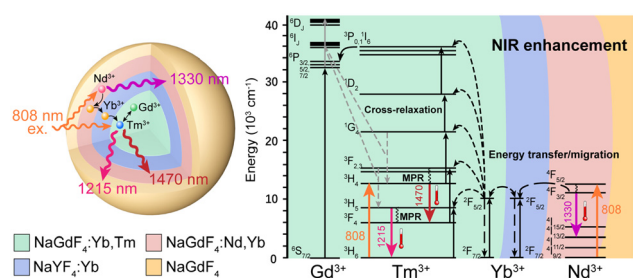
Scheme 1 Schematic of the NaGdF 4 :Yb,Tm@NaYF 4 :Yb@NaGdF 4 :Yb,Nd@NaGdF 4 nanocomposite as a dual ratiometric luminescence nanothermometer (DRLNT). Under the excitation of an 808 nm light source, Nd 3+ ions and Tm 3+ ions are activated to generate near infrared (NIR) emissions. With the cross-relaxation and phonon-assisted energy transfer processes among lanthanide ions, NIR emissions of DRLNT can be enhanced. The emission at 1215 nm generated from Tm 3+ is used as a reference and the emissions at 1470 and 1330 nm from Tm 3+ and Nd 3+ serve as working wavelengths for temperature sensing.
