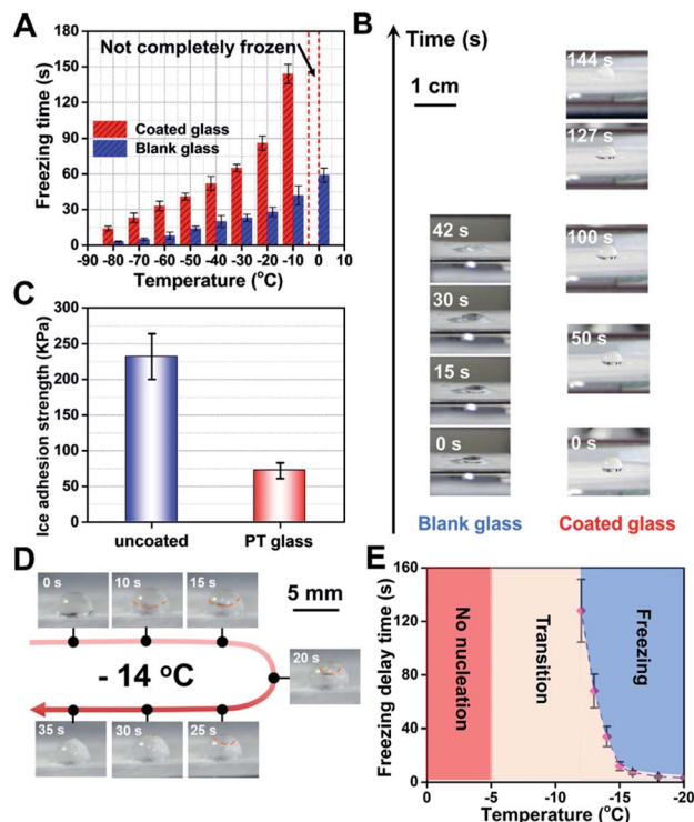
Fig. 4 (A) The freezing time of 5 \mu\text{L} droplets under different ambient temperature conditions. (B) The process of 5 \mu\text{L} droplets freezing on the surface of coated glass and blank glass at -10 °C. (C) Ice adhesion strength of blank glass and photothermal coating. (D) The process of 5 \mu\text{L} droplet freezing under light conditions at an ambient temperature of -14 °C. (E) Time taken for droplets to freeze completely under different room temperature conditions at one solar illumination.
