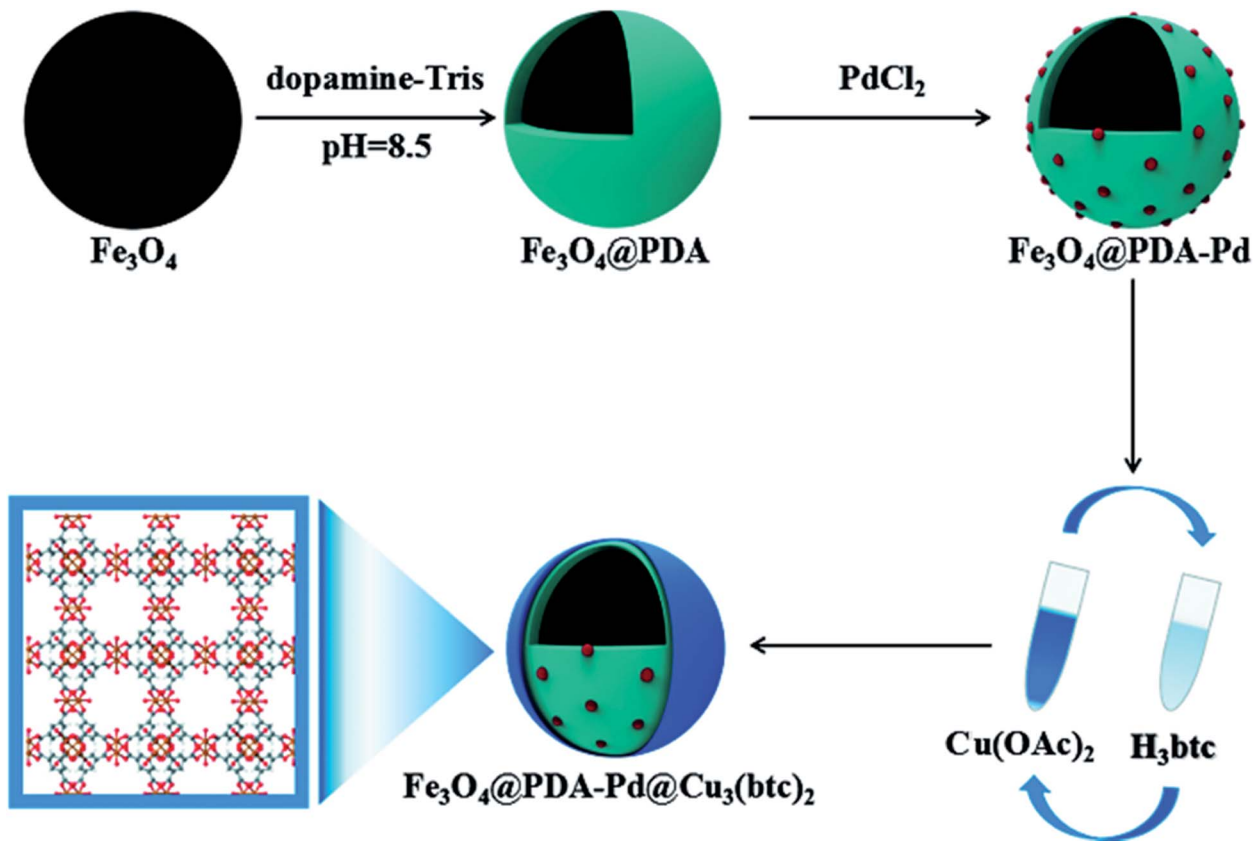
Fig. 9 Schematic of the procedure for the synthesis of the \text{Fe}_3\text{O}_4@\text{PDA-Pd}@\text{[Cu}_3(\text{BTC})_2] nanocomposite. This figure was adapted with permission from ChemCatChem , 2018, 10, 1446–1454. 77
