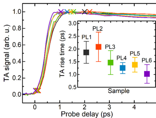
Fig. 6 Initial part of the transient absorption response to a short-pulse (250 fs) excitation of six samples with the increasing doping level in the samples from PL1 to PL6. The inset shows the rise times (see the text for their definition) for the samples.
