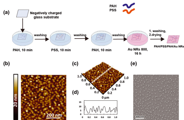
Fig. 3 Functionalization of glass substrates with Au NR 800. Schematic of the procedure used to modify a glass substrate with a polyelectrolyte multilayer (PEM) and incorporation of Au NR 800 by dipping (a). Topographical analysis of the Au NR 800-modified glass substrate by AFM (b) along with the corresponding three-dimensional topographic image (c) and the analysis of the line profile (d). Morphological characterization of a representative Au NR 800-functionalized substrate performed by SEM (e).
