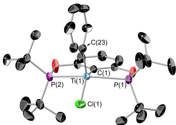
Fig. 8 ORTEP plot of 6 . Thermal ellipsoids at 50% probability, hydrogens omitted for clarity. Selected bond lengths (Å) and bond angles ( ^\circ ): Ti(1)–P(1) 2.6109(6), Ti(1)–P(2) 2.6109(6), Ti(1)–C(1) 2.2129(19), Ti(1)–C(23) 2.100(2), Ti(1)–Cl(1) 2.3157(6), P(1)–Ti(1)–P(2) 143.72(2), C(1)–Ti(1)–Cl(1) 144.36(5).
