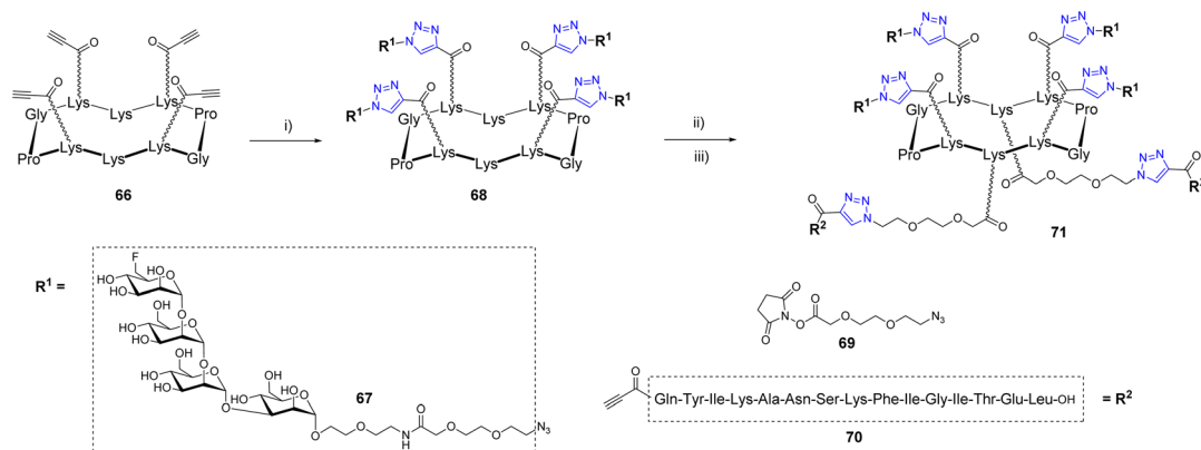
Scheme 13 Structure of an oligomannose-based glycocluster prepared by successive CuAAC reactions. Reagents and conditions: (i) 67 , CuSO 4 , sodium ascorbate, t -BuOH/H 2 O (1 : 1), approx. 90%; (ii) 69 , 0.05 M NaHCO 3 , CH 3 CN/MeOH (1 : 1); (iii) 70 , CuSO 4 , sodium ascorbate, t -BuOH/H 2 O (1 : 1), 70%.
