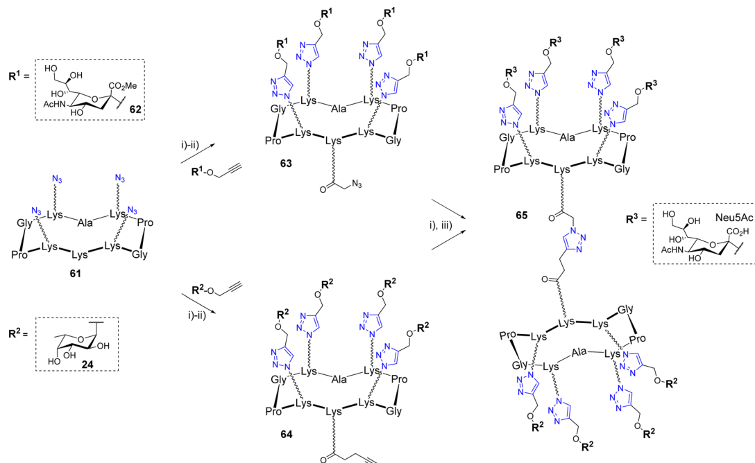
Scheme 12 Synthesis of fucosylated and sialylated heteroglycocluster 65 . Reagents and conditions: (i) CuSO 4 ·5H 2 O, THPTA, sodium ascorbate, DMF/PBS (pH 7.5) (1 : 1), r.t., 1 h, 79% for 63 , 85% for 64 , 71% for 65 ; (ii) N -succinimidyl azidoacetate or N -succinimidyl pentynoate, DIPEA, DMF, r.t., 2 h, quant.; (iii) LiOH, r.t., 2 h, quant.
