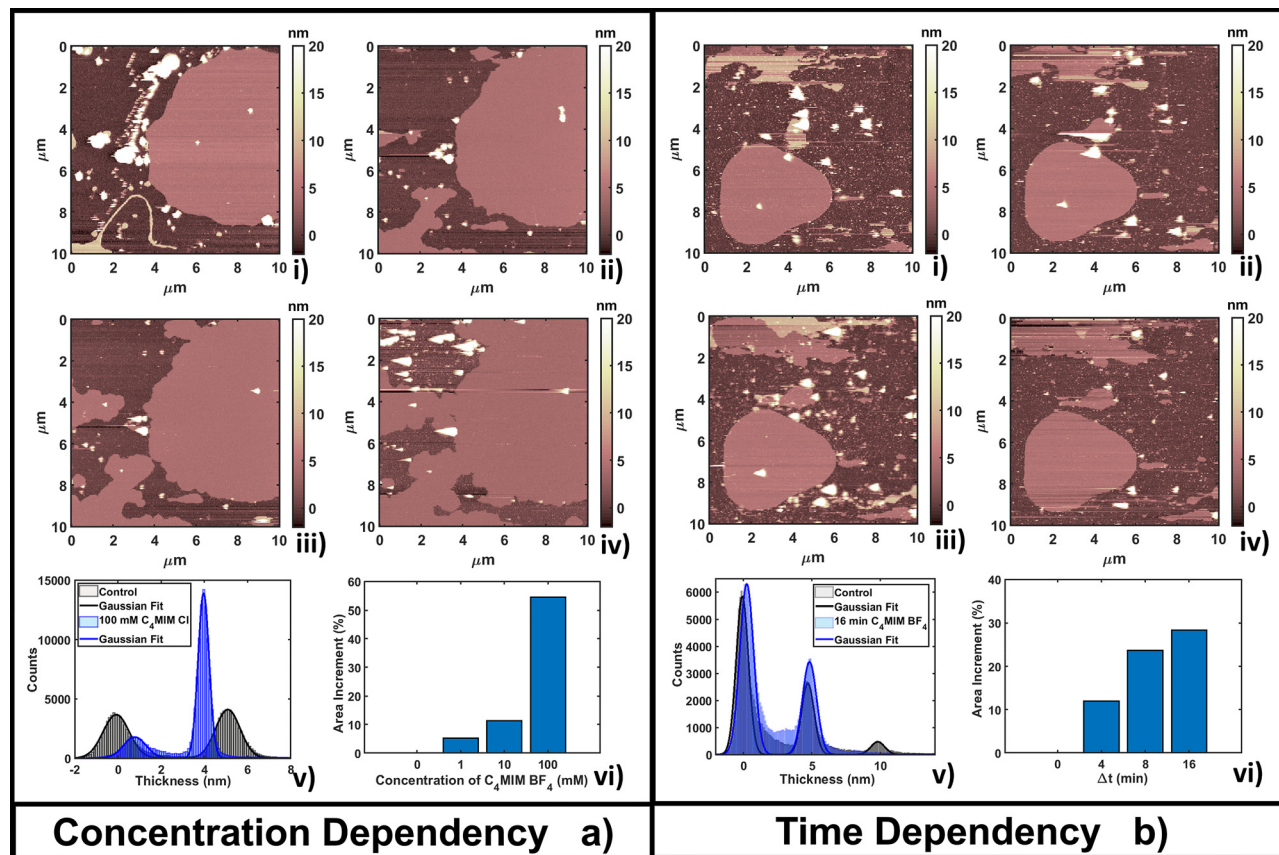
Fig. 2 Evolution of a DOPC bilayer as a result of (a) adding increasing concentrations of [C 4 MIM][BF 4 ] at fixed time of measurements T = 4 min after the interaction and (b) fixing the concentration at 10 mM and observing the time evolution. In all images bright colors represent amorphous liquid-like aggregates and darker regions represent the substrate. In panel (a), image (i) represents the control, (ii) 1 mM, (iii) 10 mM and (iv) 100 mM concentration. (v) Quantitative height histogram relative to the first and last frame; (vi) area increment (%) of the single bilayer referenced on the control. In panel (b), image (i) represents the control, (ii) 4 min, (iii) 8 min and (iv) 16 min of interaction with 10 mM [C 4 MIM][BF 4 ]. (v) Quantitative height histogram relative to the first and last frame; (vi) area increment (%) of a single bilayer referenced on the control.
