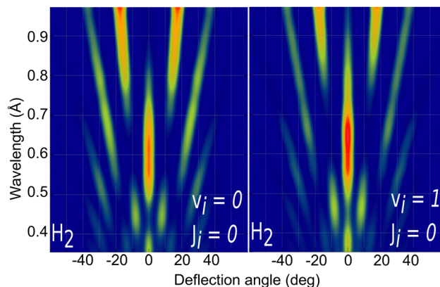
Fig. 4 Simulated \text{H}_2/\text{KCl}(001) GIFMD patterns along the crystallographic direction [100] for the initial rovibrational state: left panel ( v = 0, J = 0 ); right panel ( v = 1, J = 0 ).
