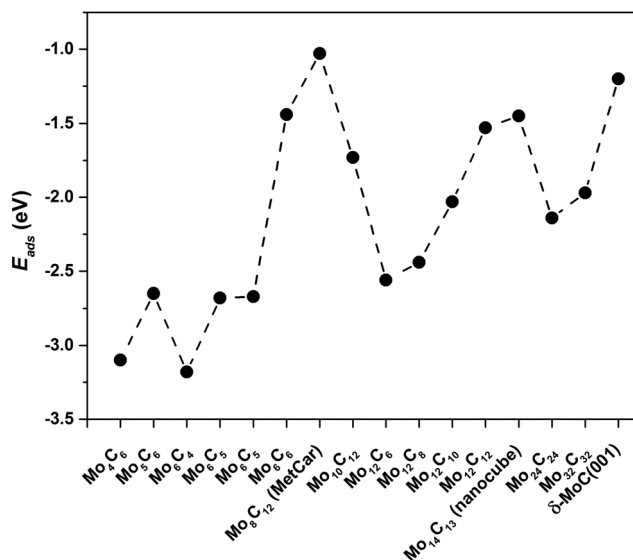
Fig. 8 \text{CO}_2 adsorption energy, E_{\text{ads}} , for the most stable \text{CO}_2 bonding mode on the different nanoparticles.
