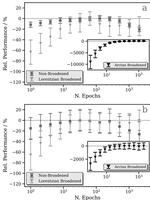
Fig. 2 Relative performance of the DNN at the Pt L 2 (a) and L 3 (b) edges as a function of the number of training cycles (‘‘epochs’’). Three models are shown, differing in their choice of target function: the target functions used are (i) the calculated absorption cross-section (without any post-processing), (ii) the calculated absorption cross-section broadened with a fixed-width Lorentzian function (FWHM = 0.5 eV), and (iii) the calculated absorption cross-section broadened with an arctangent convolution model (see Theory and computational details). Data points are averaged over 100 K-fold cross-validated evaluations; error bars indicate one standard deviation.
