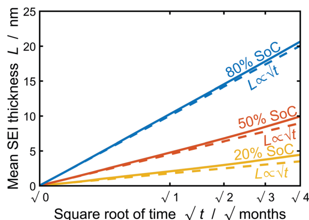
Fig. 2 Growth of the mean SEI thickness \bar{L}_{\text{SEI}} = 1/A_x \int_0^{x_x} L_{\text{SEI}} d\bar{x} over the square root of storage time \sqrt{t} . Different colors indicate different states of charge. Dashed lines indicate a \sqrt{t} -growth for comparison.
