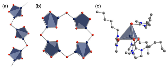
Fig. 3 Infinite zig-zag-strand structure of the anion 1\text{D}-\{[\text{Hg}_2\text{Te}_4]^{2-}\} (a), molecular structure of the heavy metal porphyranoid anion [\text{Hg}_8\text{Te}_{16}]^{8-} (b), molecular structure of the cationic complex [(\text{C}_6\text{C}_1\text{ImTe})_4\text{Hg}]^{2+} (c). Hydrogen atoms are omitted for clarity. Color code: Hg-dark blue, Te-red, C-grey, N-blue.
