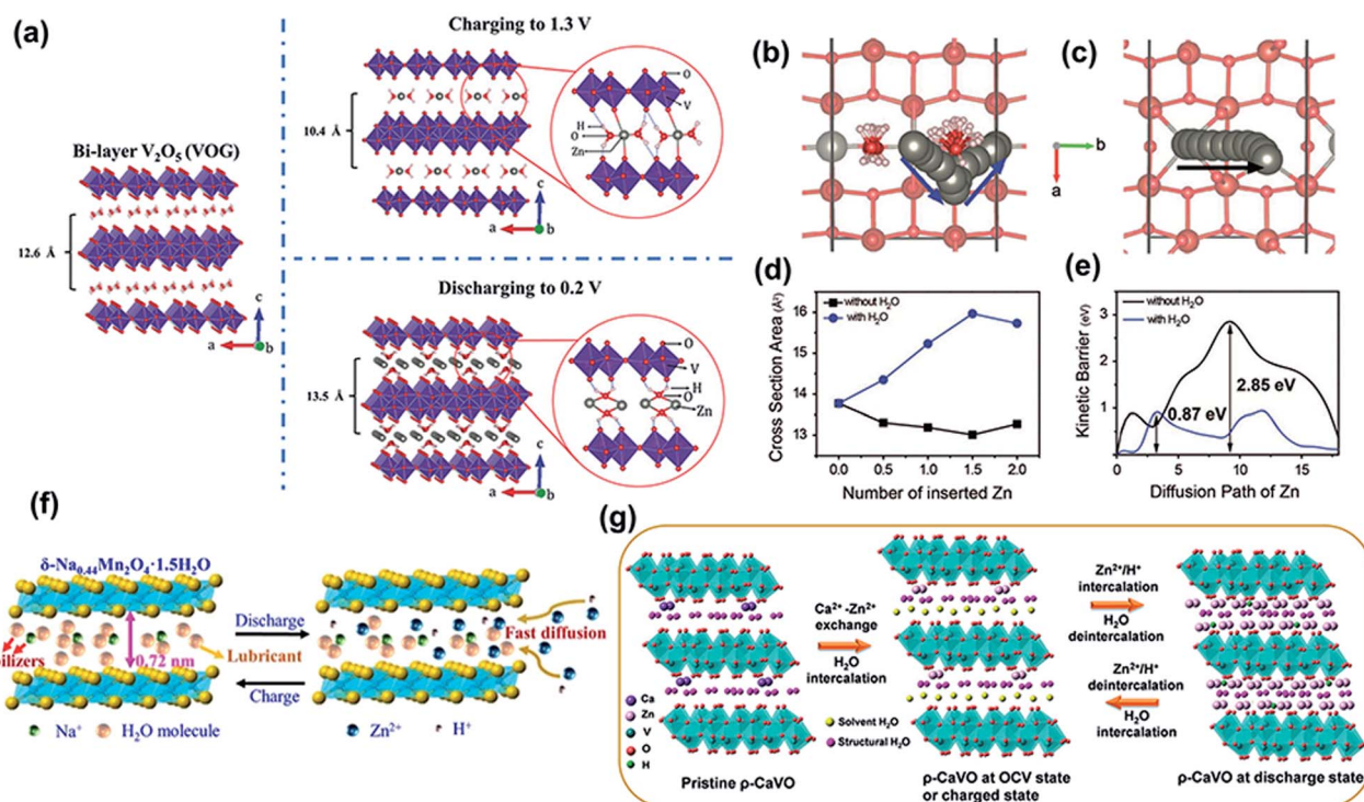
Fig. 3 (a) The proposed crystal structures of pristine V 2 O 5 ·nH 2 O, and V 2 O 5 ·nH 2 O after charging to 1.3 V, and discharging to 0.2 V. Reproduced with permission. 47 Copyright 2017, Wiley-VCH. Diffusion paths of Zn ions (b) with and (c) without water (projected down [001]). (d) Change in the cross-sectional area of the diffusion path during Zn intercalation with and without water. (e) Calculated diffusion barriers for paths in (b) and (c). (b–e) Reproduced with permission. 72 Copyright 2019, Wiley-VCH. (f) Schematic of Na ion and water molecule pre-intercalated δ-MnO 2 for Zn ion storage. Reproduced with permission. 76 Copyright 2019, American Chemical Society. (g) Schematic illustration of the reaction mechanism of p-CaVO. Reproduced with permission. 78 Copyright 2019, American Chemical Society.
