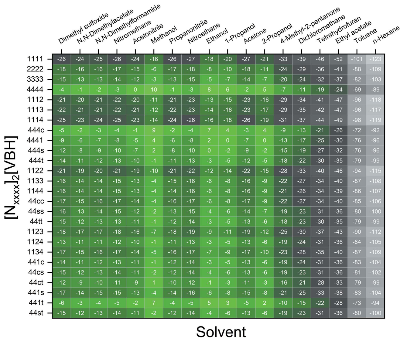
Fig. 7 Heat map of \log(S_0) for [N_{xxx}]_2[VBH] in different solvents. Solubilities were taken relative to the solubility of [N_{444}]_2[VBH] in MeCN. Green cells indicate better or comparable solubilities with respect to [N_{444}]_2[VBH] in MeCN.
