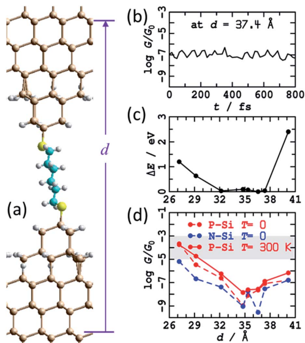
Fig. 3 Modelling the STMBJ experiment assuming regular H-terminated silicon tips form on each electrode. (a) 2D (3 × 3) model of two flat Si(111)-H surfaces with two added H-terminated Si layers in the shape of a tip, spanned by S(CH 2 ) 6 S, at d = 36.6 Å; Si-brown, S-yellow, C-cyan, H-white. (b) Conductivity at zero voltage evaluated along a 800 fs MD trajectory for P-type silicon. (c) Average energy of each MD simulation. (d) Conductivity at zero voltage for P-type and N-type silicon for static geometries ( T = 0 K) and averaged over T = 300 K MD trajectories; the shaded region shows the observed conductance found throughout extensions of 3–10 Å for P-type Si at 300 K. See ESI† Fig. S2 and S3 for more information.
