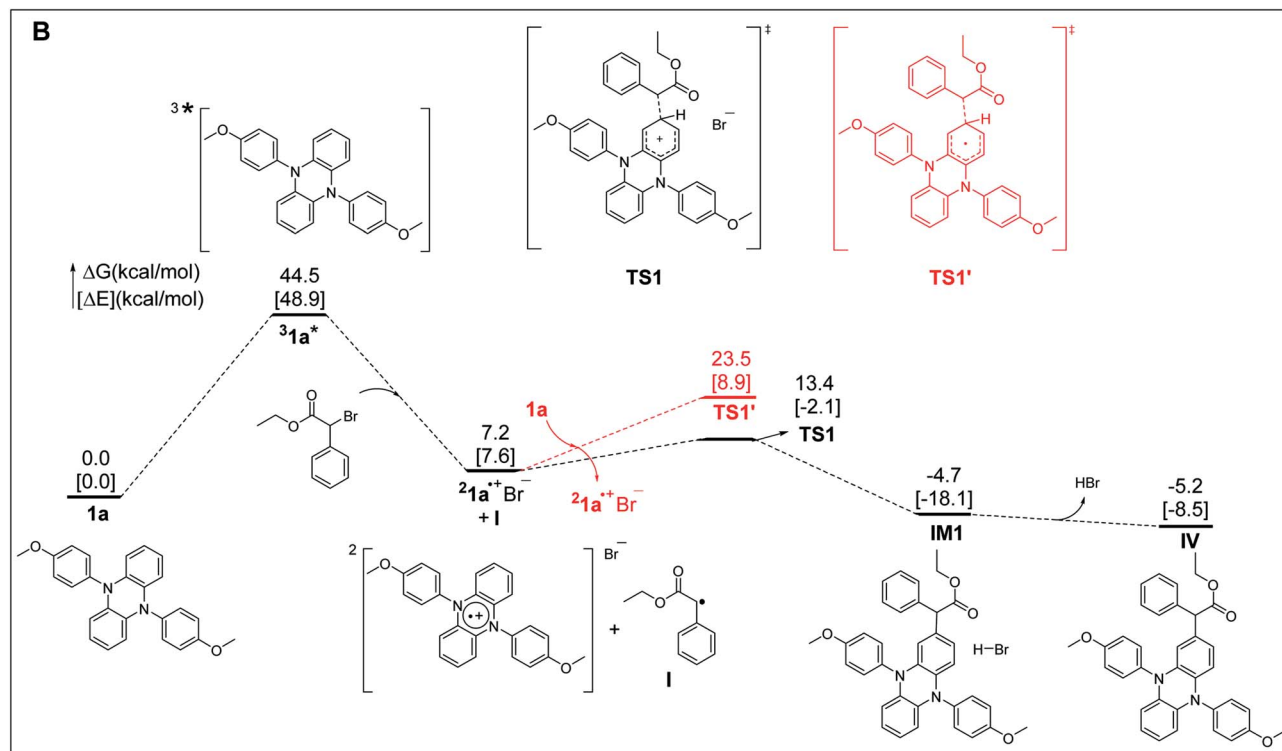
Fig. 4 Mechanistic investigations. (A) Control experiments. (B) Computed Gibbs energy profile ( \Delta G in kcal mol -1 ) and electronic energy [ \Delta E ] in brackets] at the BP86+D3(BJ)/def2-TZVPP (CPCM, SOL = DMAC)//BP86+D3(BJ)/def2-SVP (CPCM, SOL = DMAC) of the reaction. The proposed mechanism is simplified as a monosubstituted core modification of 1a .
