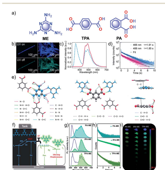
Fig. 6 (a) Chemical structure of ME , TPA and PA . (b) Photographs of emission (top) and phosphorescence (bottom) of the ME-IPA cocrystal. (c) Steady-state photoluminescence (blue dotted line) and phosphorescence (red line) spectra along with (d) phosphorescence decay of the emission bands at 466 and 488 nm, respectively, of ME-IPA . (e) Molecular packing of ME-IPA showing intermolecular interactions from the same plane with ME as the center and IPA as the center along with ME and IPA with adjacent planes. (f) Schematic of TADF-assisted transfer from ME to IPA enhancing the RTP lifetime. (g) Prompt and delayed fluorescence spectra and corresponding (h) time-resolved fluorescence decay profiles, and (i) photographs showing the long-afterglow of ME-PA , ME-IPA , and ME-TPA . Reproduced with permission from (a–e) ref. 91 (copyright 2018, American Chemical Society) and (f–h) ref. 77 (copyright 2019, WILEY-VCH).
