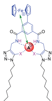
Fig. 6 Schematic representation of through-bond (TB, blue) and through-space (TS, green arrows) interactions that drive anion recognition in the cationic state of 1.XB/HB in solution and at 2.XB/HB SAM . In the more polar solvent environment of high dielectric the TS contribution is diminished and TB contributions are significant. In the low dielectric SAM environment, TS contributions are strongly enhanced such that binding in the cationic state is switched-on more strongly, inducing a larger sensor response.
