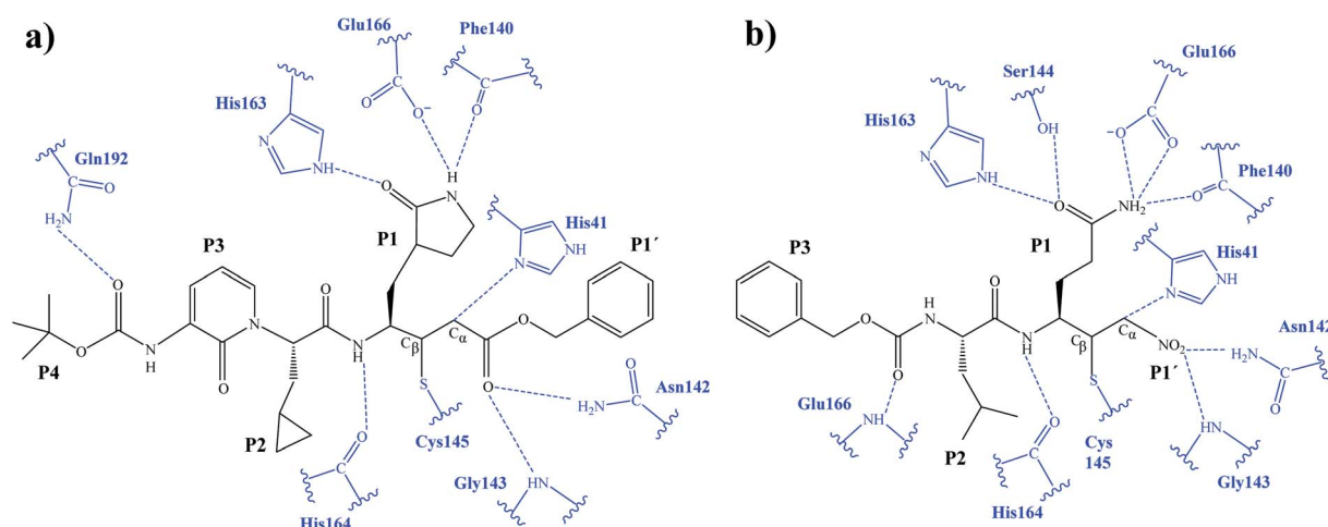
Fig. 5 Schematic representation of the active site in the E-I complex and details of the H-bond interactions between the inhibitor and the active site of the SARS-CoV-2 M^{pro} from QM/MM MD simulations of compound B1 (a) and compound B2 (b).
