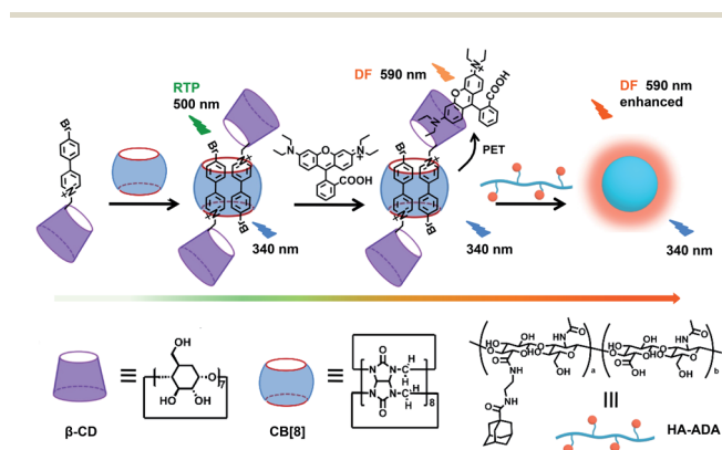
Scheme 1 Construction of the supramolecular assembly for a purely organic light-harvesting PET system and related molecules.
